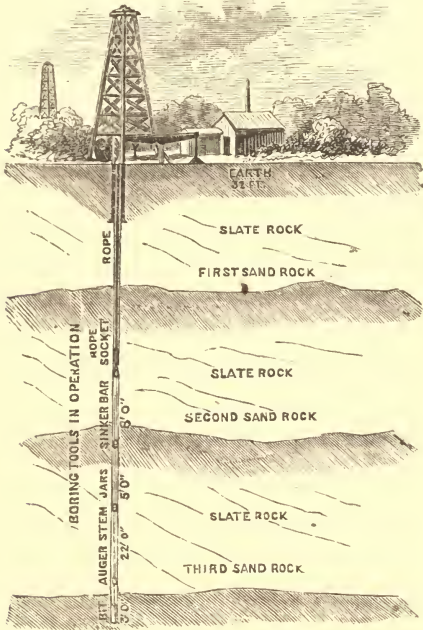
Boring Tools in Operation—Pennsylvania Oil Region.
